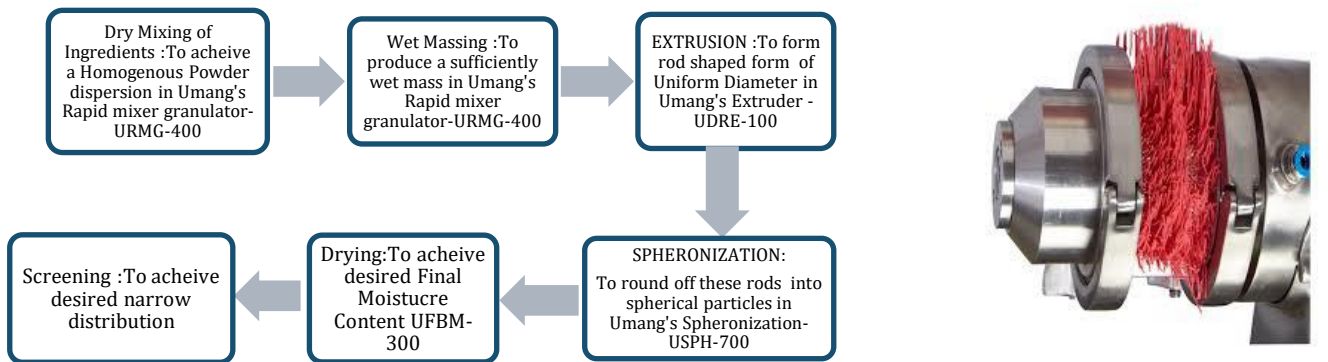
UDRE-100 Umang Pharmatech Extruder
